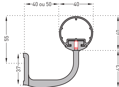
55 mm bugled self-locking aluminium bracket silver anodised effect (overall projection 80 mm or 90 mm on request)
