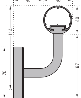
Swan-neck with 70 mm rose self-locking brushed stainless steel bracket (overall projection 80 mm)
