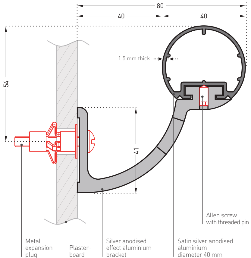
60 mm full self-locking aluminium bracket silver anodised effect (overall projection 80 mm)
