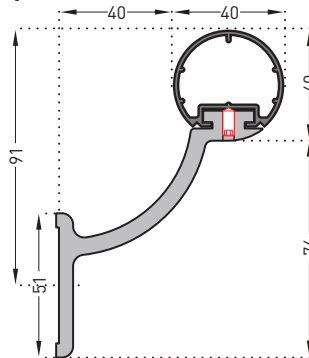
60 mm full self-locking aluminium bracket silver anodised effect (overall projection 80 mm)
